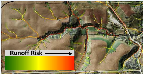
Figure 2. High runoff risk/concentrated flow areas identified using the stream power index tool.
