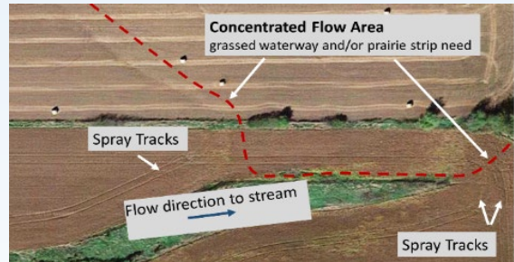
Figure 3. Avoid pesticide applications in concentrated flow areas by installing grassed waterways.
